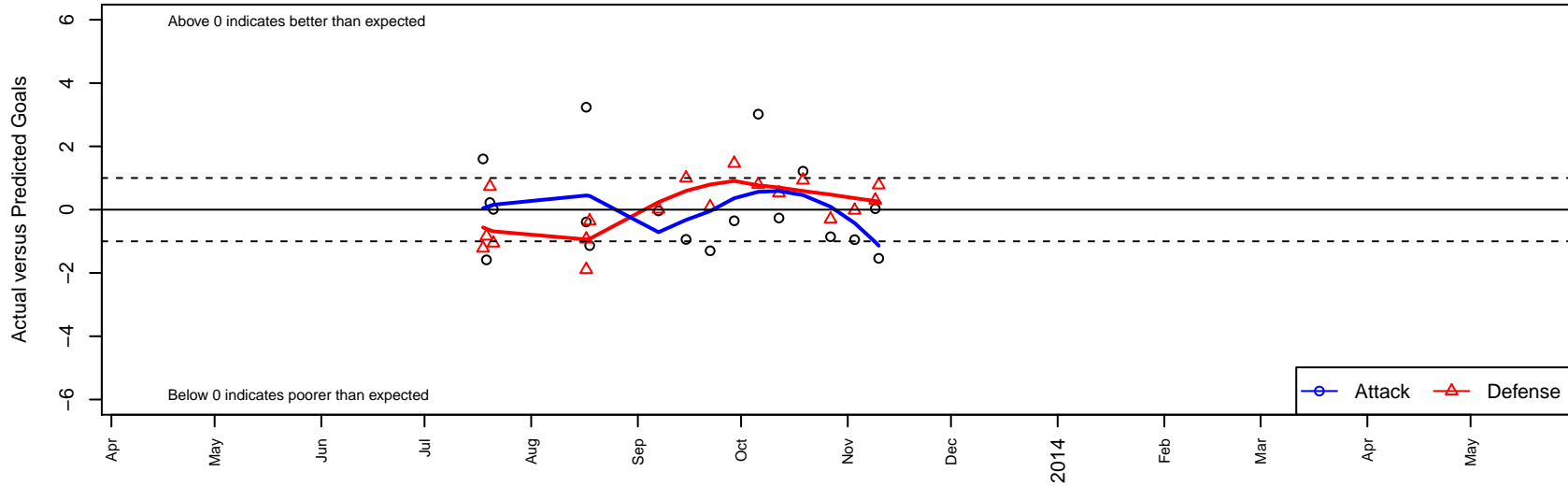
Carlsbad Elite B95 Dots are actual minus expected GF (blue circles) and GA (red triangles). Blue line is smoothed change in attack strength. Red is smoothed change in defense strength.
